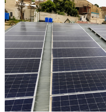
Surabhi Woollen , Bikaner, Rajasthan (50 kWp 2020)
