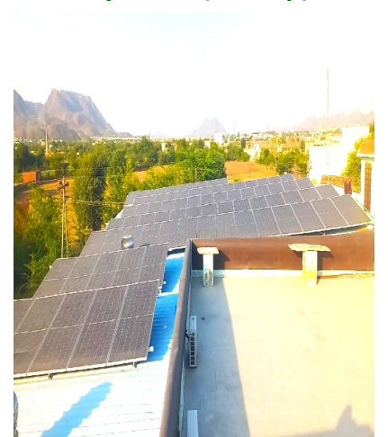
Bal Gopal Foods, Ajmer Rajasthan (50 kWp)
